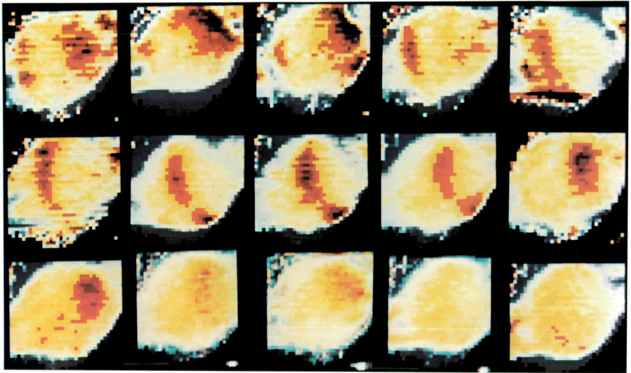
Figure 1. Spectral images of Saturn obtained with the SPIFI + SIT vidicon at a spatial resolution of better than 2". Here proper spatial sampling was observed, with each pixel corresponding to 0.65" in the original images. The grey scale indicates the presence of CH 4 absorption in the rotational feature of CH 4 at 6196.82Å, which we have studied extensively in the laboratory. The band which appears and moves across the image of the ball of Saturn (the rings are not plotted) reflects the Doppler shift of the absorption in the narrow pass band of the SPIFI. From this "cube" of images (there are a total of 27) we can construct more than 1000 spectral profiles on the disc of the planet, and many more for the rings.
